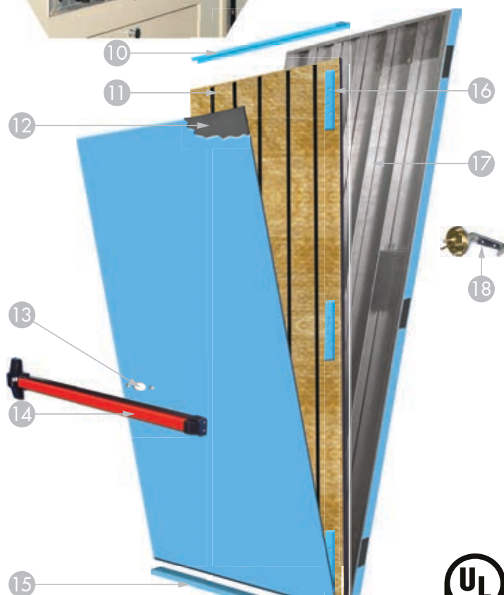
Fire Doors
